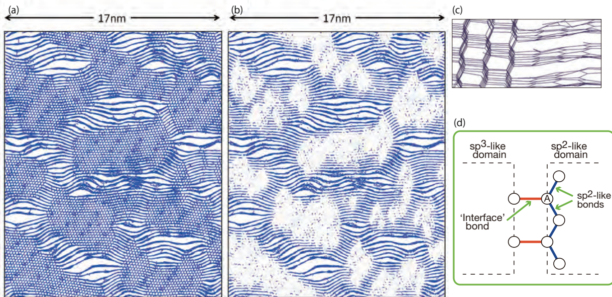
Figure 3: Nano-domain analysis of sp^2 - sp^3 nano-composite carbon solid (NCCS) visualized with the COHP or \pi COHP analysis [4]. The sp^2 (graphite-like) and sp^3 (diamond-like) domains are visualized in (a), while only the sp^2 -like domains are visualized in (b). A closeup of a sp^2 - sp^3 domain boundary is shown in (c). The atoms at a typical domain boundary are shown in (d).
